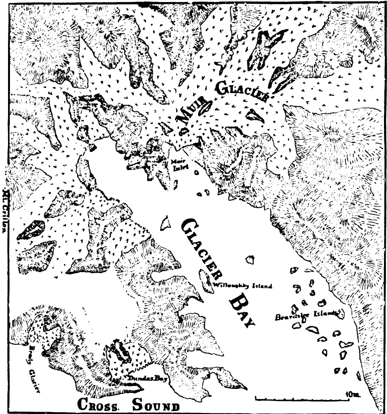
FIG. 20.—Map of Glacier Bay, Alaska, and its surroundings. Arrow-points indicate glaciated area.
